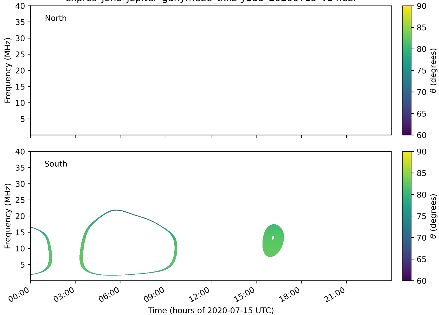
expres_juno_jupiter_ganymede_txka-y235_20200715_v14.cdf
