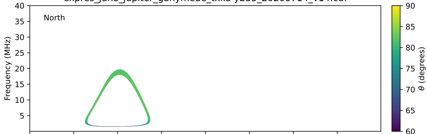
expres_juno_jupiter_ganymede_txka-y235_20200714_v14.cdf
