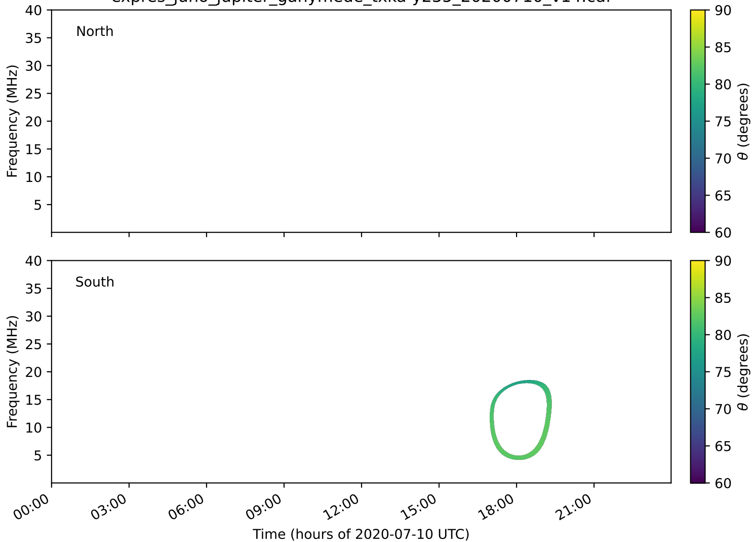
expres_juno_jupiter_ganymede_txka-y235_20200710_v14.cdf
