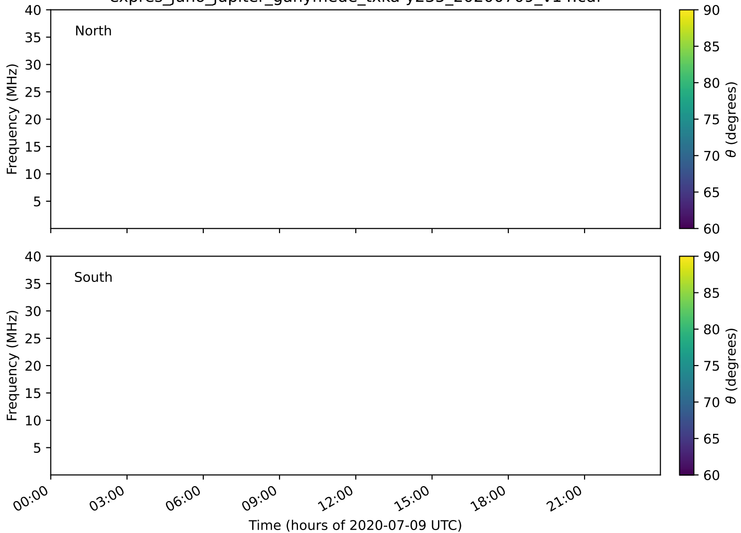
expres_juno_jupiter_ganymede_txka-y235_20200709_v14.cdf
