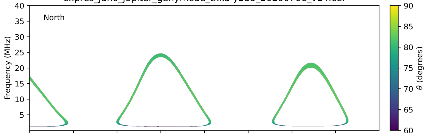
expres_juno_jupiter_ganymede_txka-y235_20200706_v14.cdf
