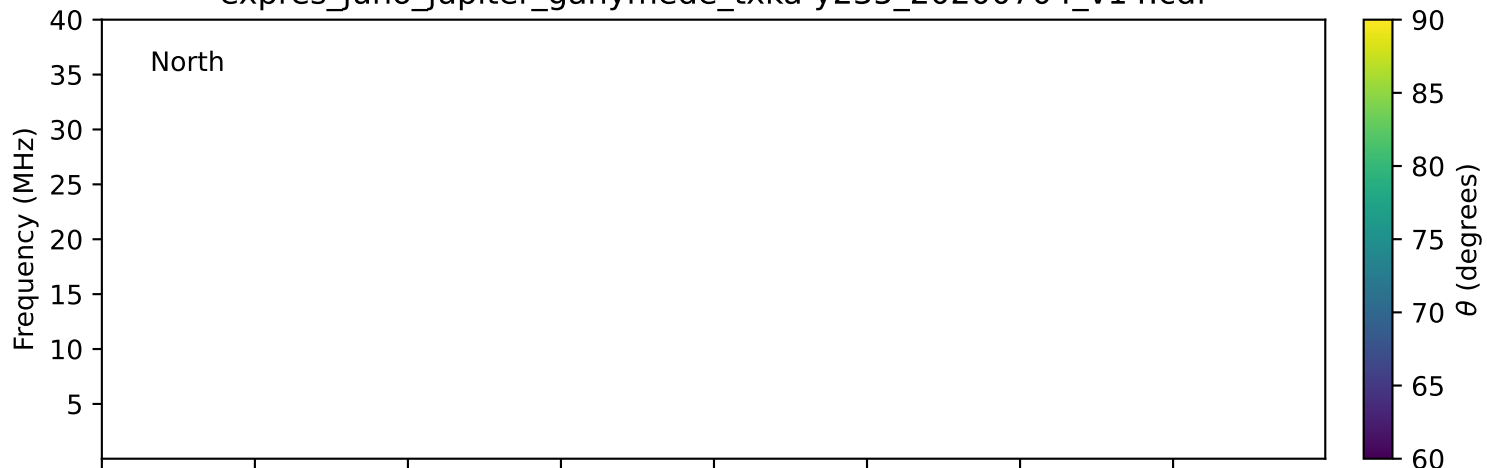
expres_juno_jupiter_ganymede_txka-y235_20200704_v14.cdf
