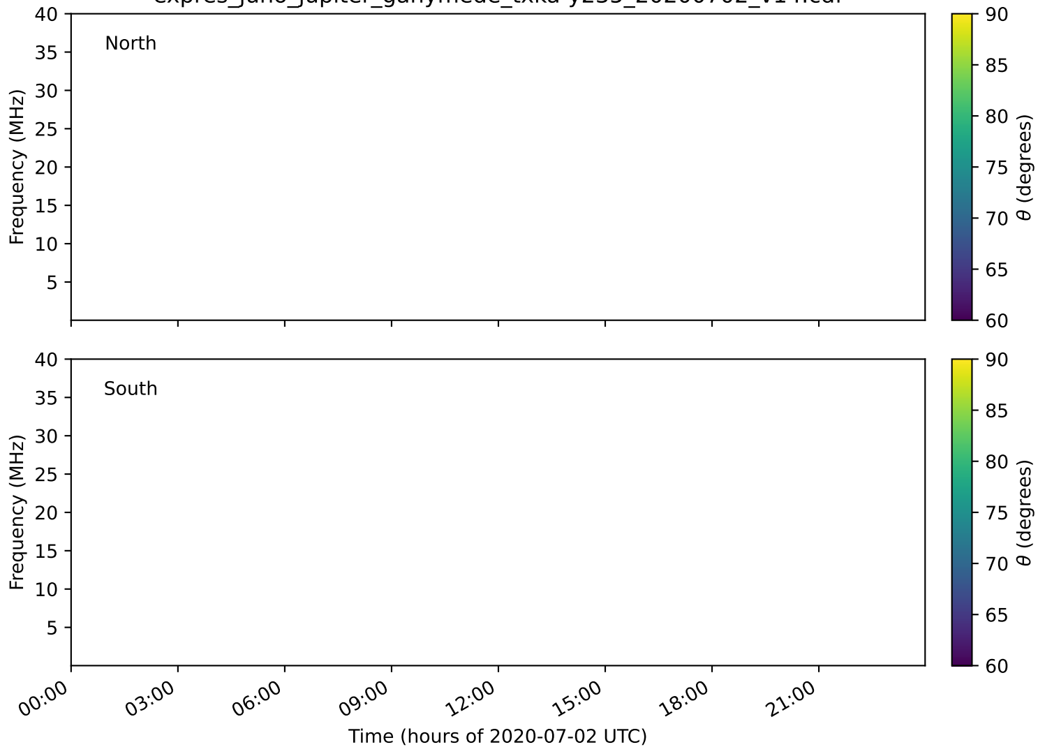
expres_juno_jupiter_ganymede_txka-y235_20200702_v14.cdf
