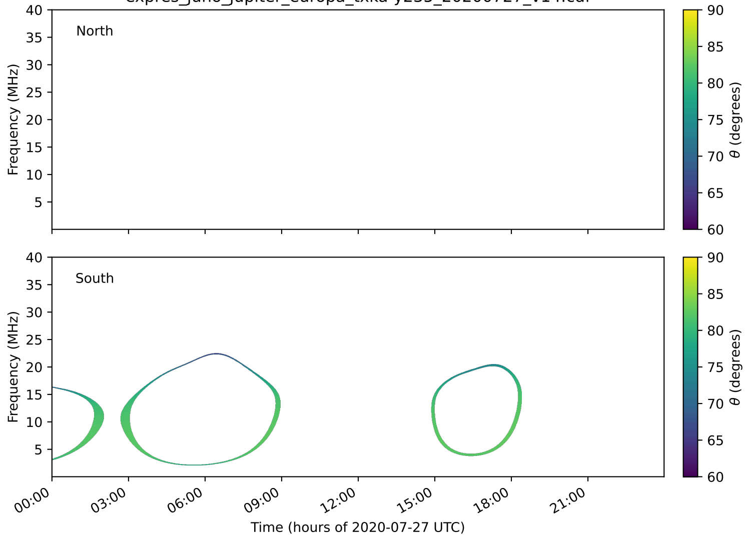
expres_juno_jupiter_europa_txka-y235_20200727_v14.cdf
