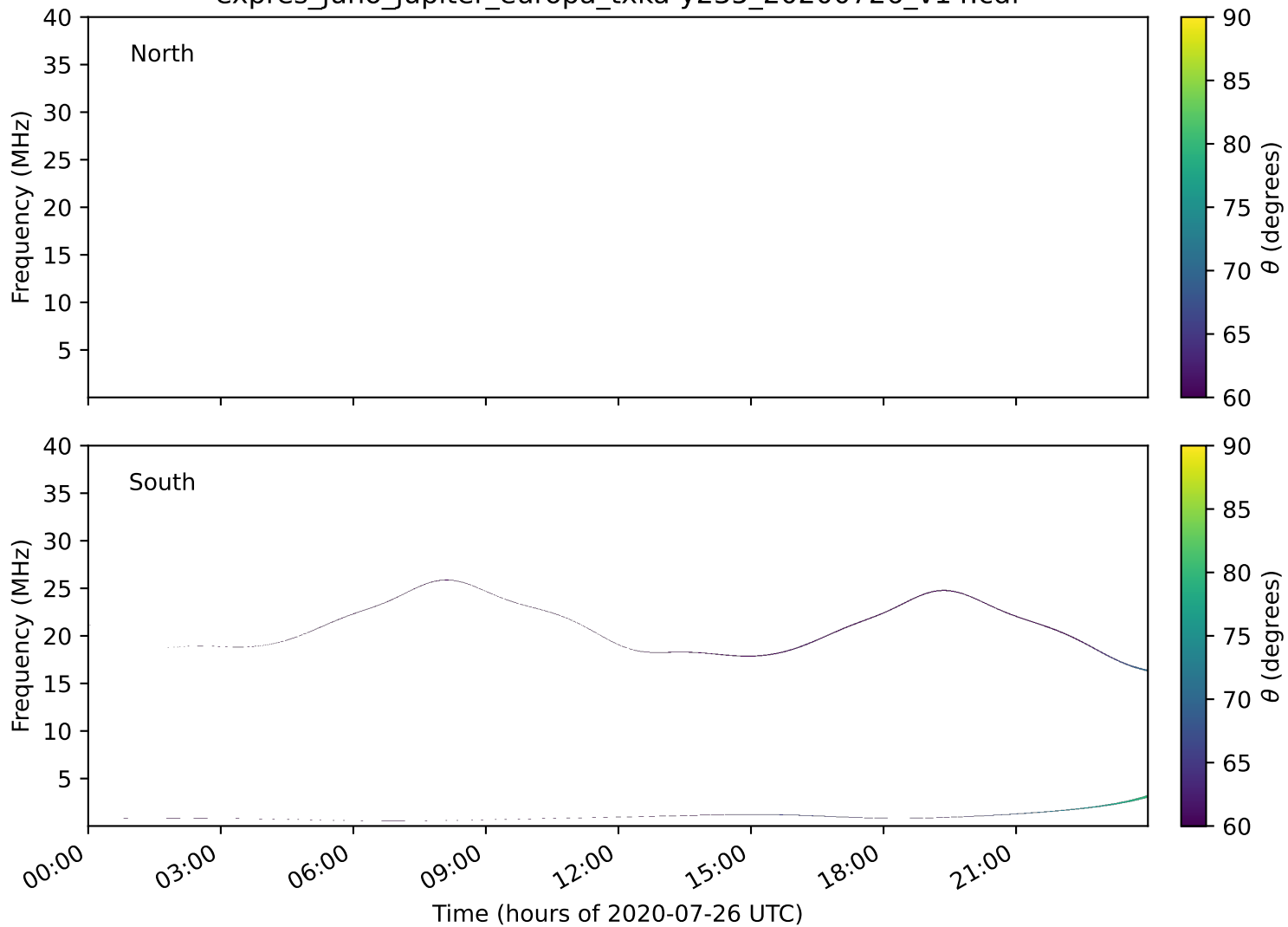
expres_juno_jupiter_europa_txka-y235_20200726_v14.cdf
