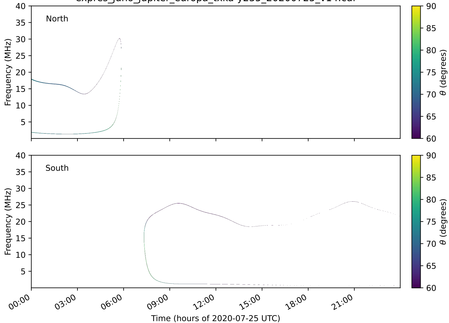
expres_juno_jupiter_europa_txka-y235_20200725_v14.cdf
