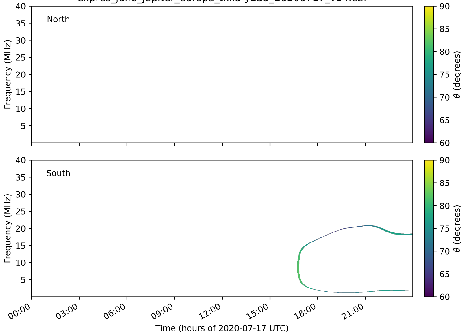
expres_juno_jupiter_europa_txka-y235_20200717_v14.cdf
