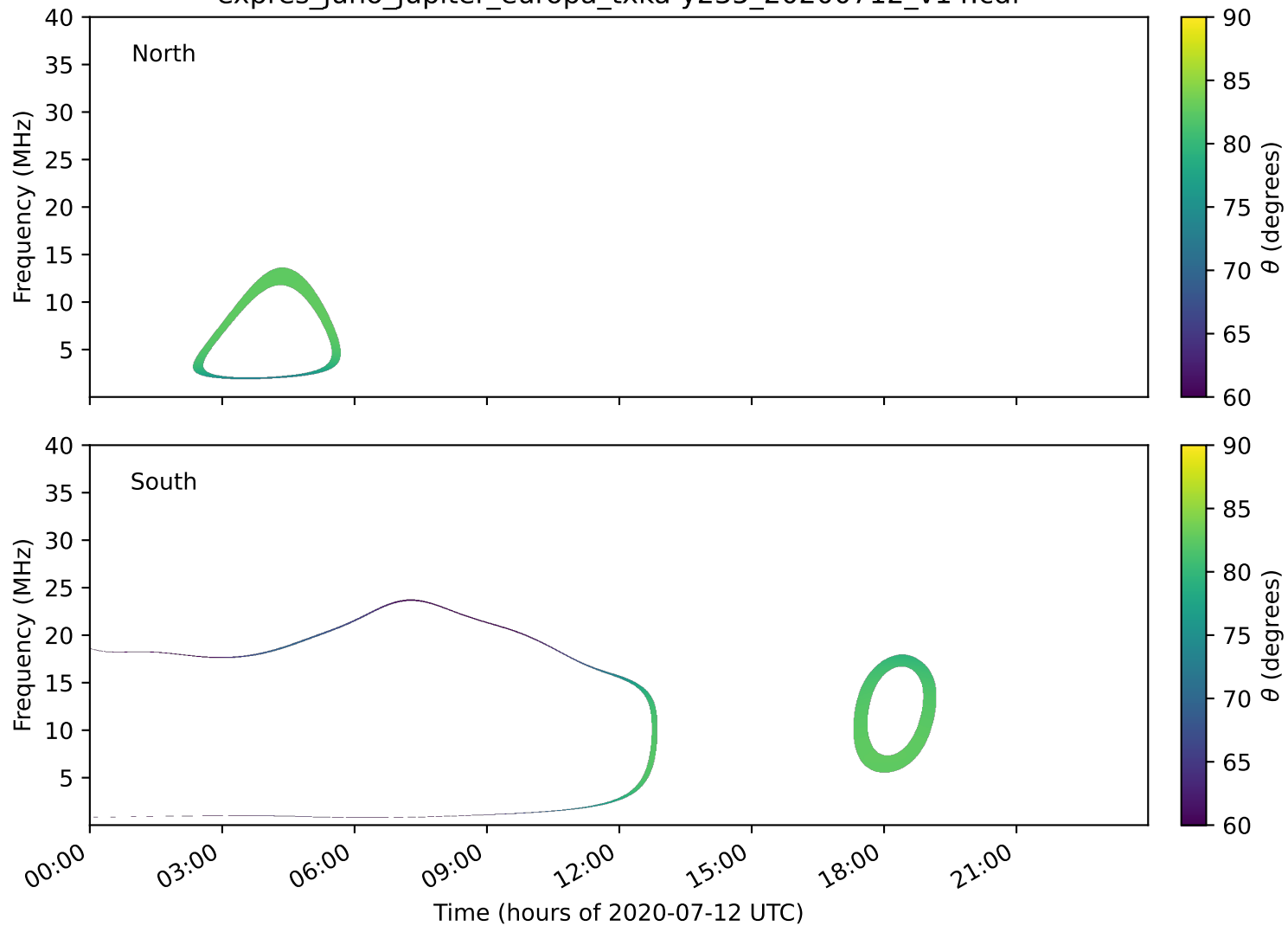
expres_juno_jupiter_europa_txka-y235_20200712_v14.cdf
