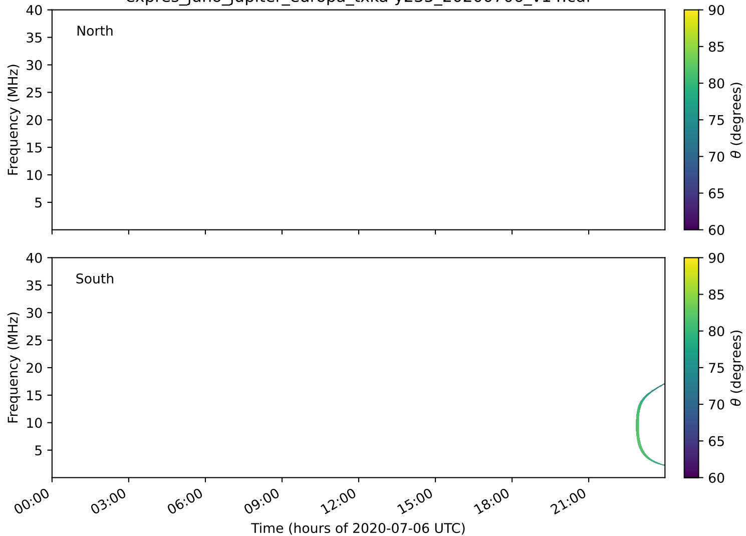
expres_juno_jupiter_europa_txka-y235_20200706_v14.cdf
