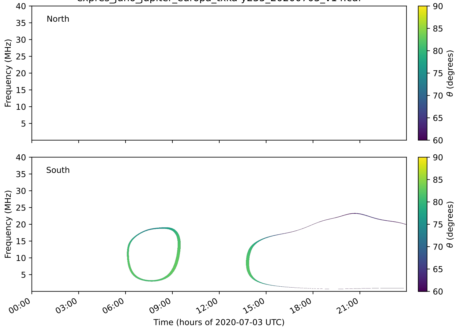
expres_juno_jupiter_europa_txka-y235_20200703_v14.cdf
