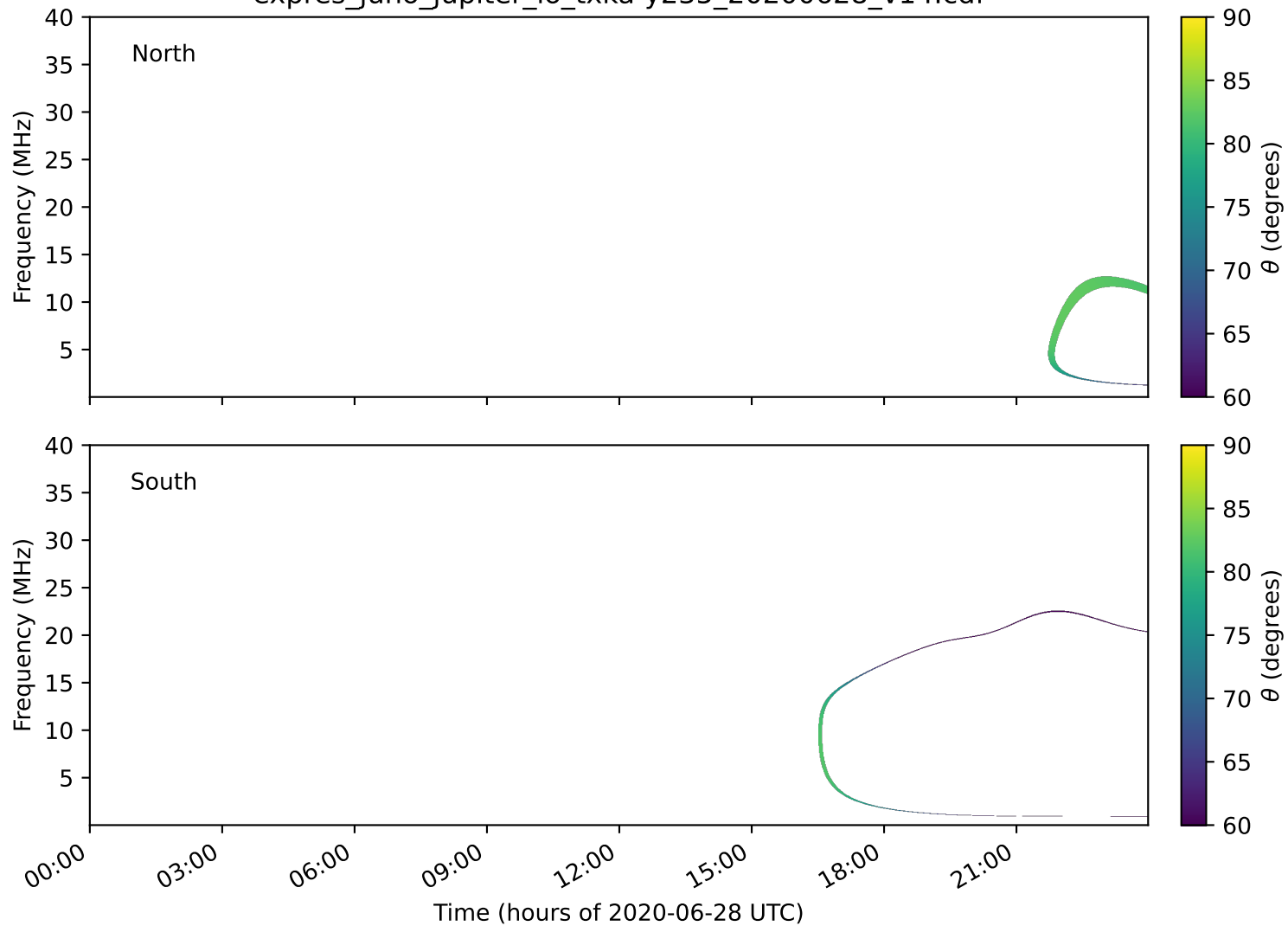
expres_juno_jupiter_io_txka-y235_20200628_v14.cdf
