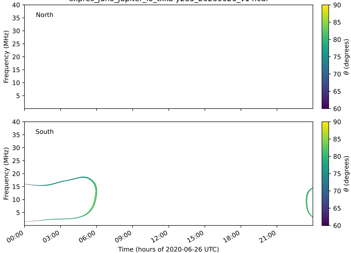
expres_juno_jupiter_io_txka-y235_20200626_v14.cdf
