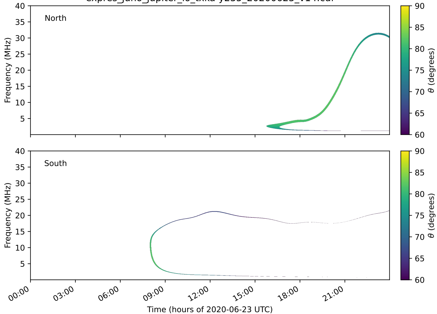
expres_juno_jupiter_io_txka-y235_20200623_v14.cdf
