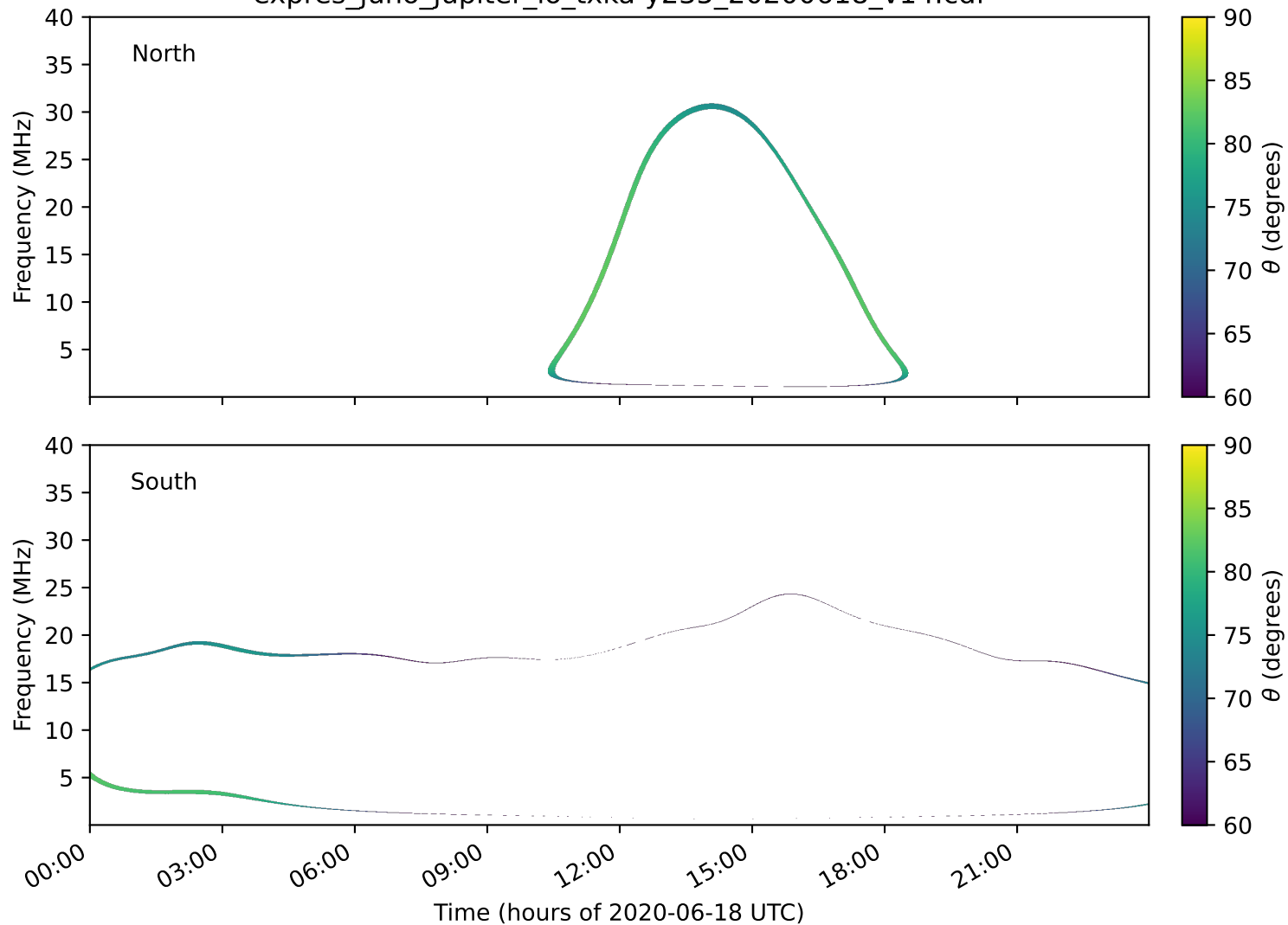
expres_juno_jupiter_io_txka-y235_20200618_v14.cdf
