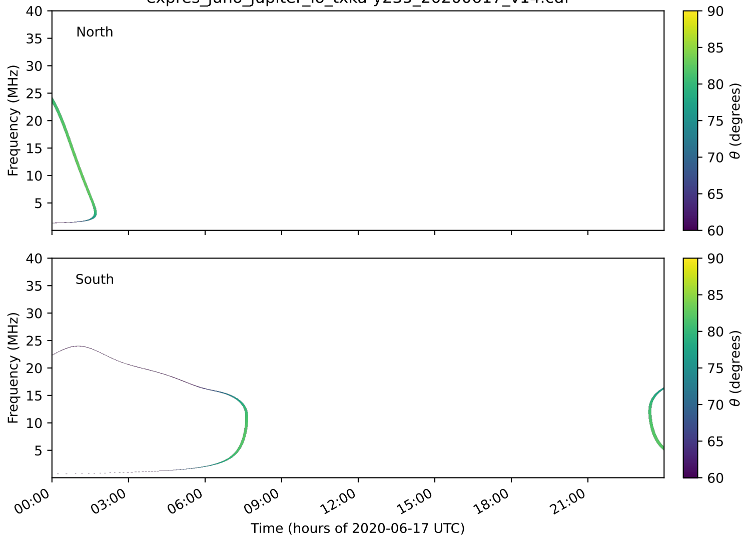
expres_juno_jupiter_io_txka-y235_20200617_v14.cdf
