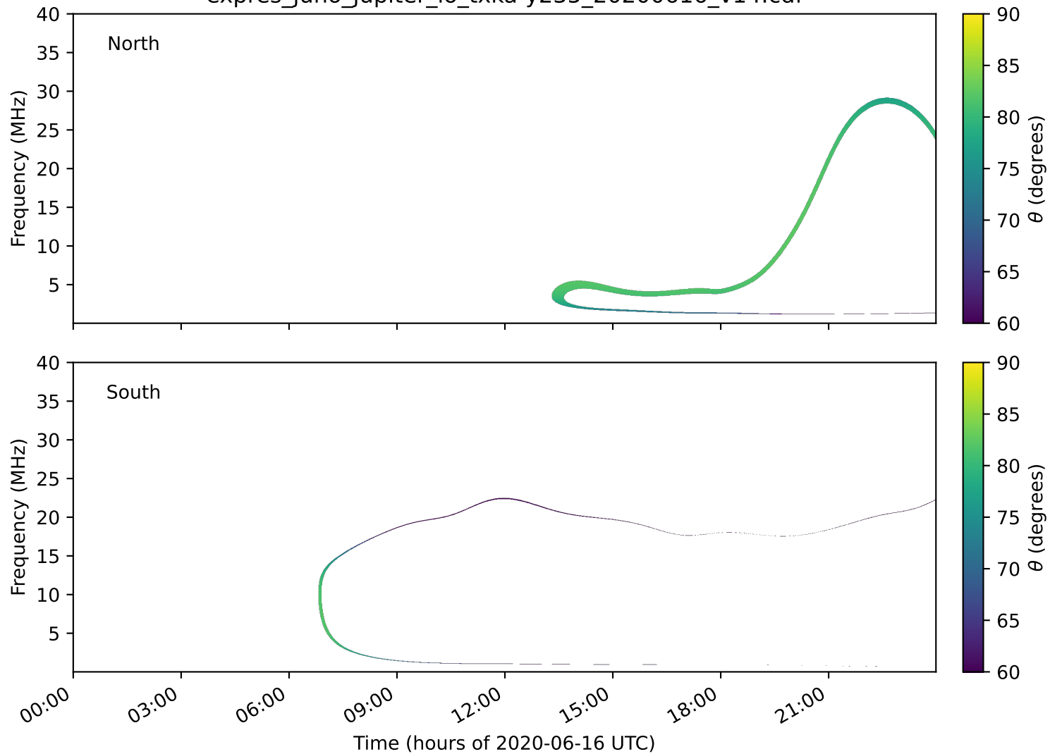
expres_juno_jupiter_io_txka-y235_20200616_v14.cdf
