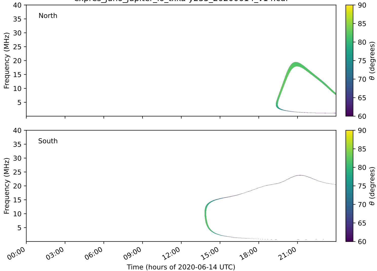
expres_juno_jupiter_io_txka-y235_20200614_v14.cdf
