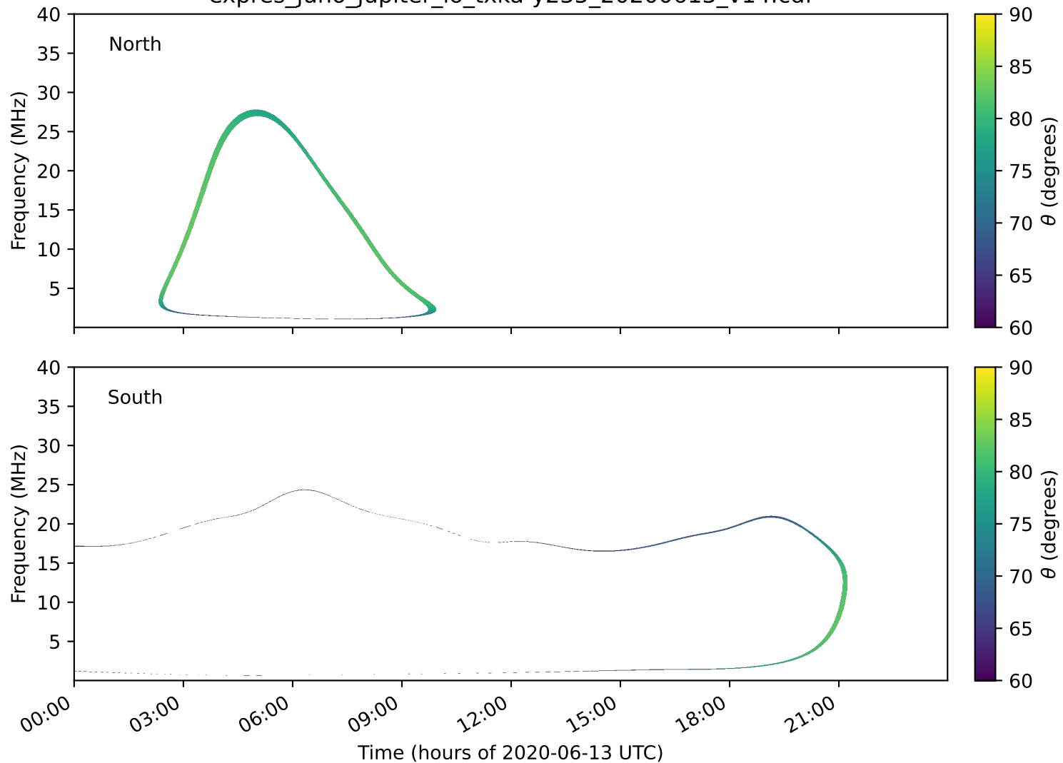
expres_juno_jupiter_io_txka-y235_20200613_v14.cdf
