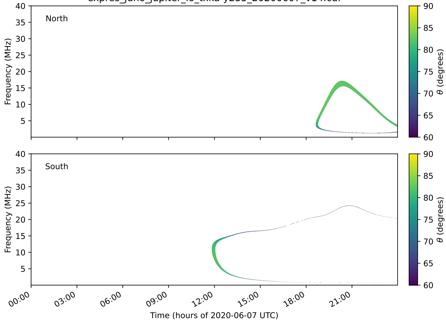
expres_juno_jupiter_io_txka-y235_20200607_v14.cdf
