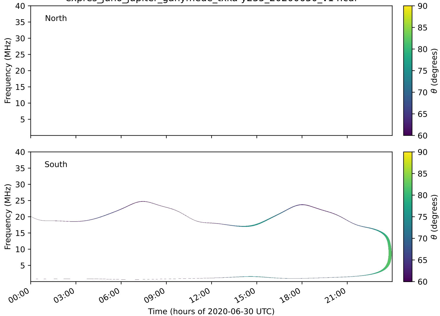
expres_juno_jupiter_ganymede_txka-y235_20200630_v14.cdf
