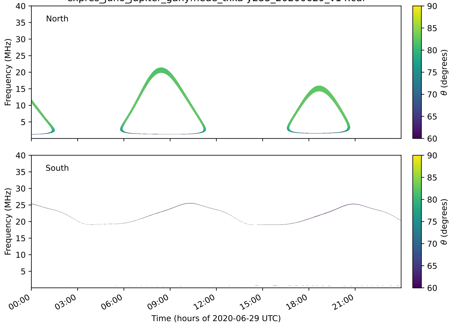
expres_juno_jupiter_ganymede_txka-y235_20200629_v14.cdf
