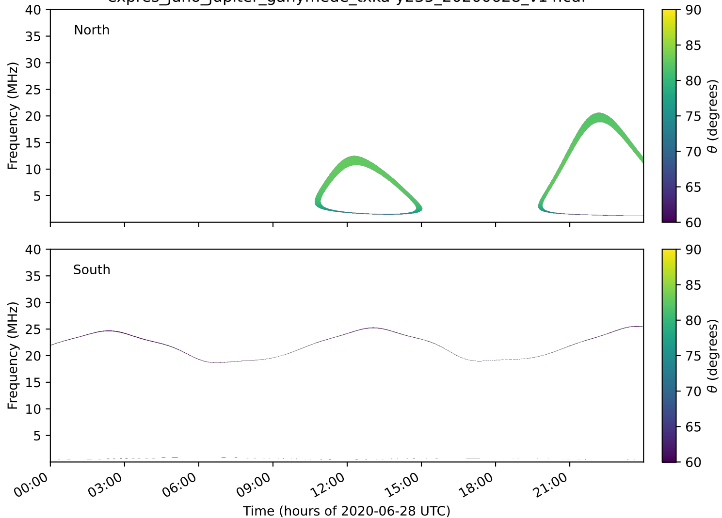
expres_juno_jupiter_ganymede_txka-y235_20200628_v14.cdf
