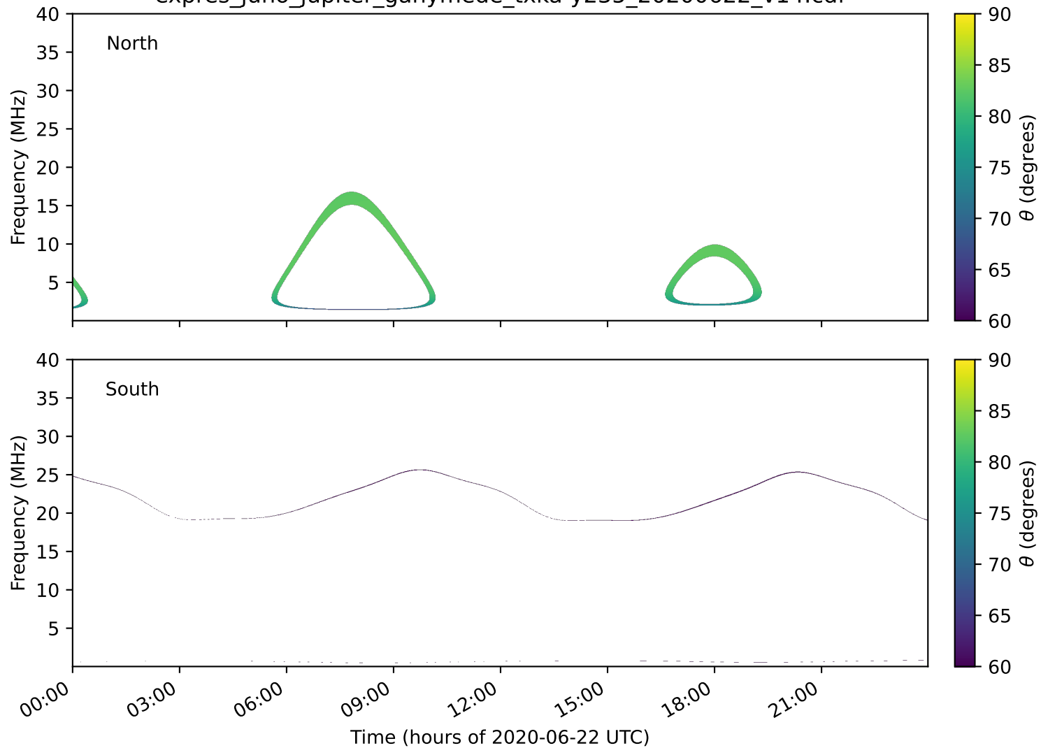
expres_juno_jupiter_ganymede_txka-y235_20200622_v14.cdf
