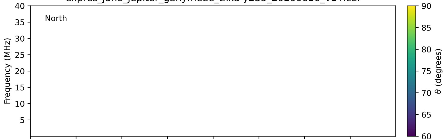
expres_juno_jupiter_ganymede_txka-y235_20200620_v14.cdf
