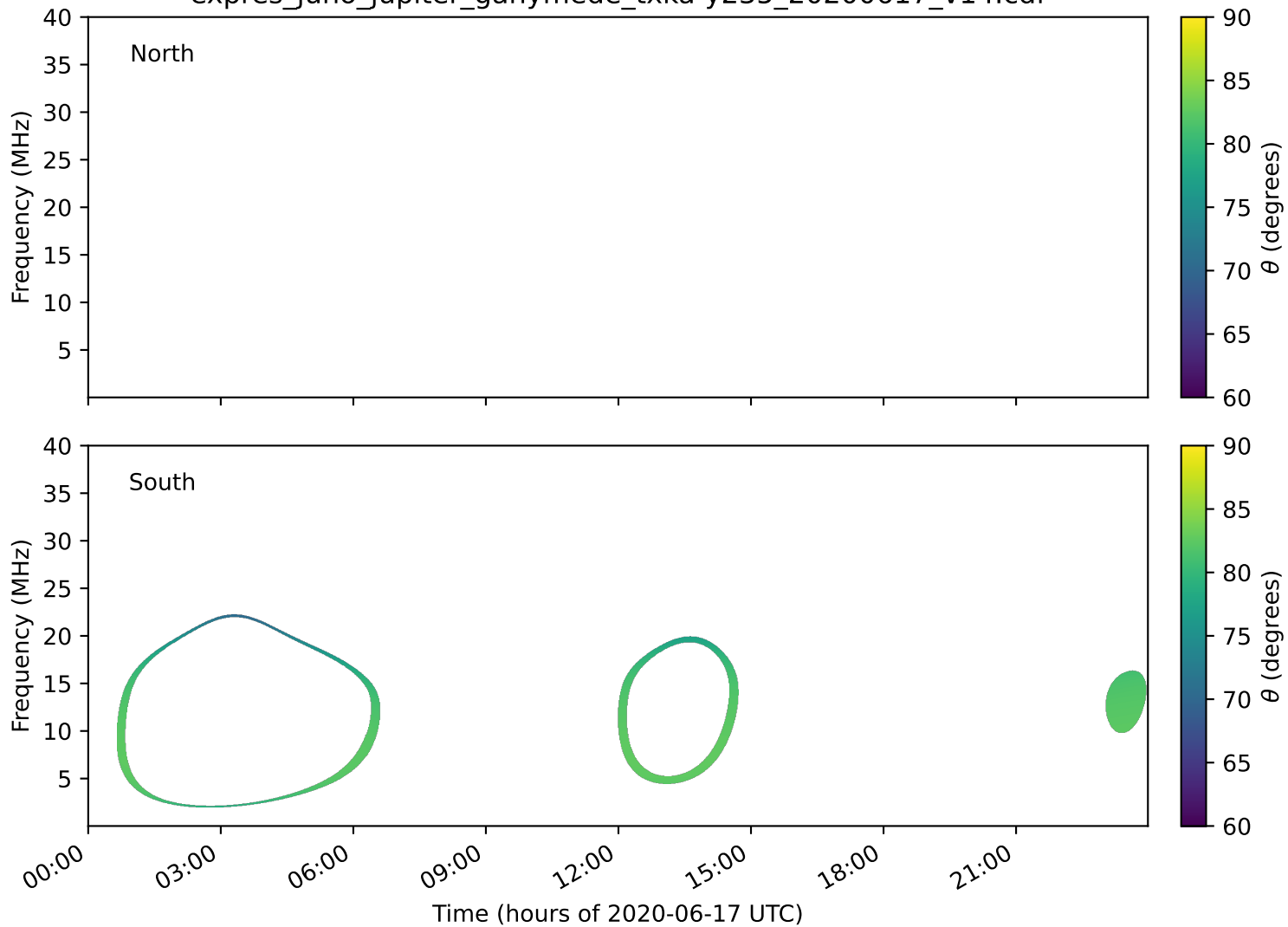
expres_juno_jupiter_ganymede_txka-y235_20200617_v14.cdf
