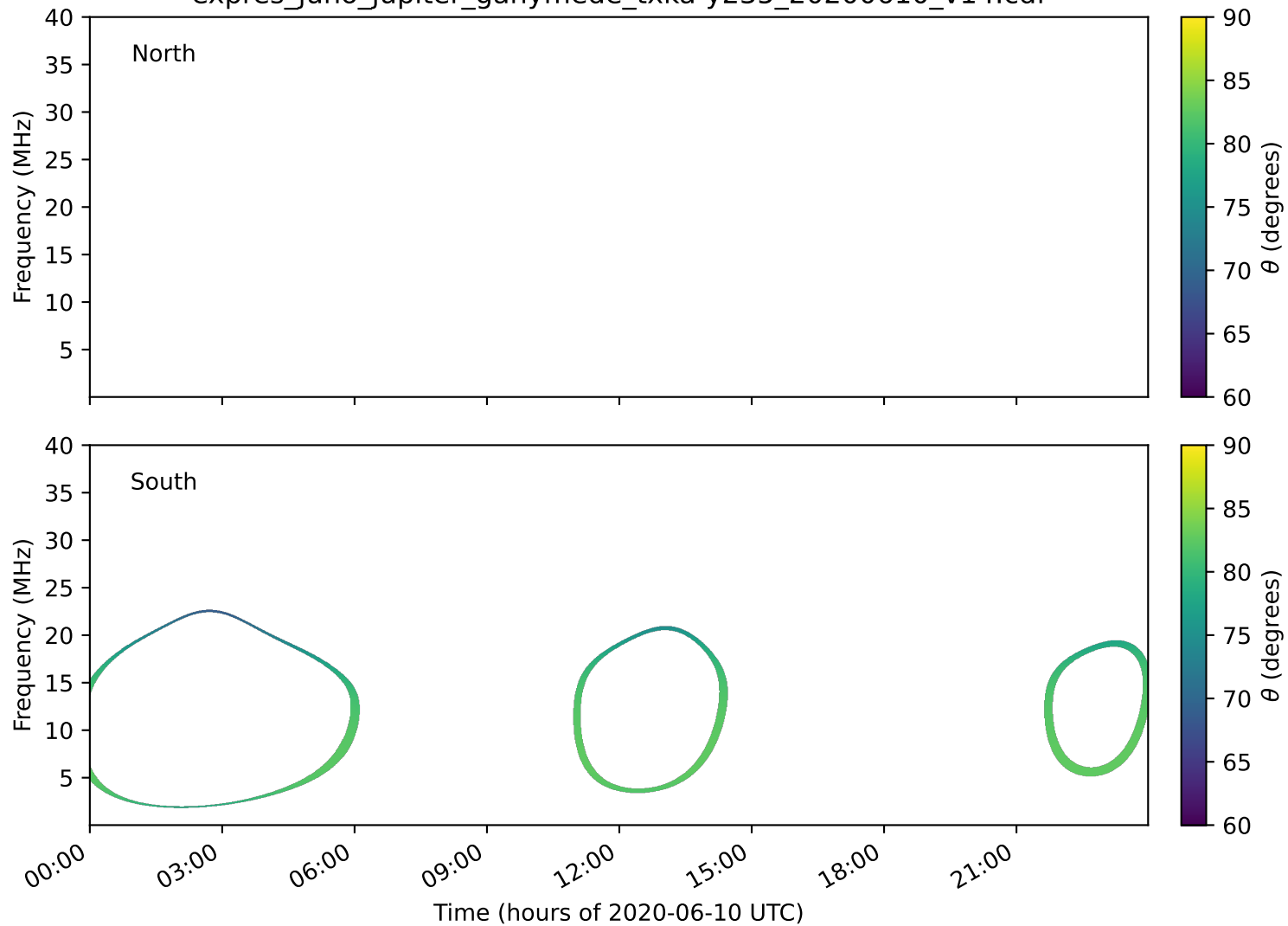
expres_juno_jupiter_ganymede_txka-y235_20200610_v14.cdf
