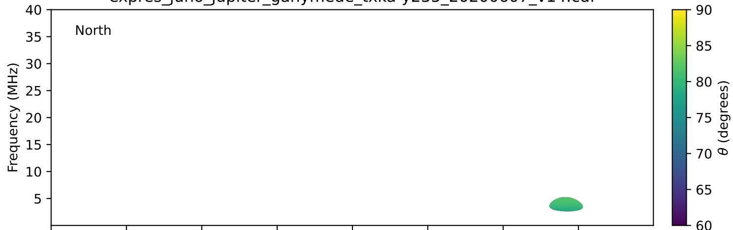
expres_juno_jupiter_ganymede_txka-y235_20200607_v14.cdf
