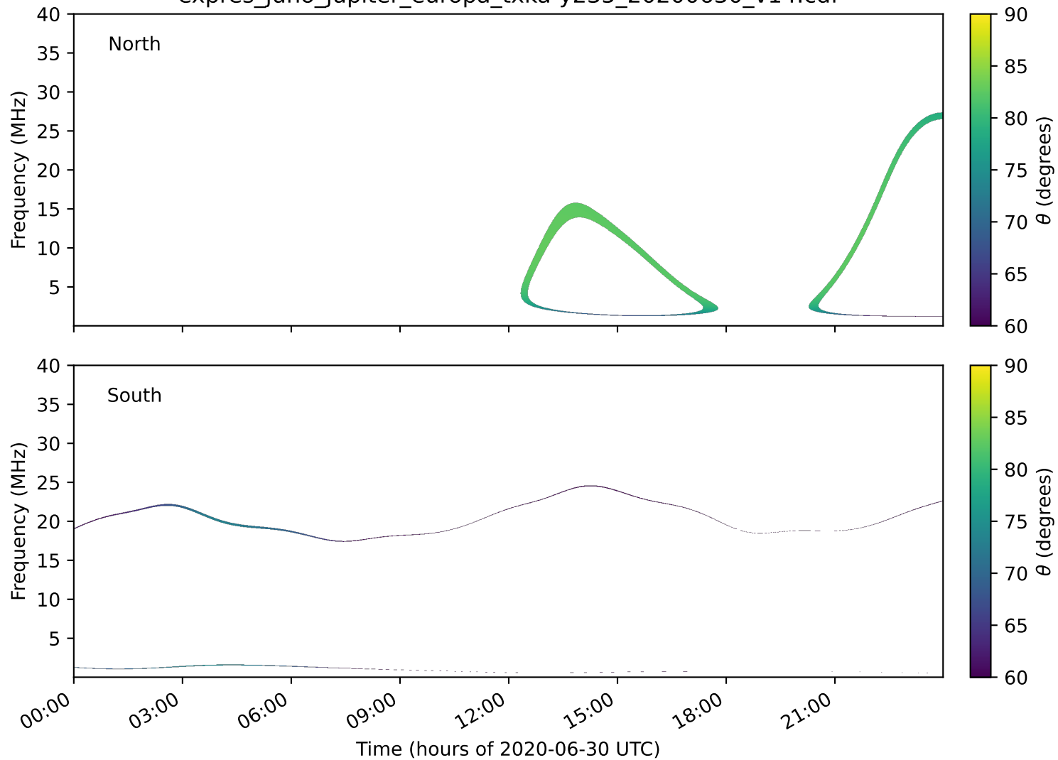
expres_juno_jupiter_europa_txka-y235_20200630_v14.cdf
