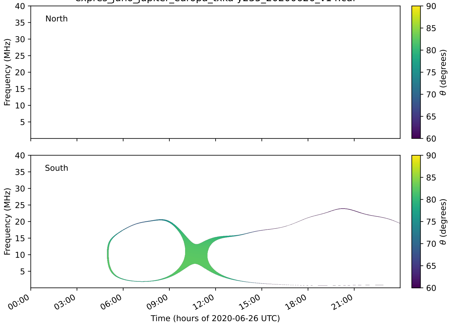
expres_juno_jupiter_europa_txka-y235_20200626_v14.cdf
