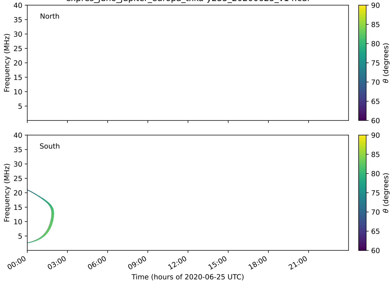
expres_juno_jupiter_europa_txka-y235_20200625_v14.cdf
