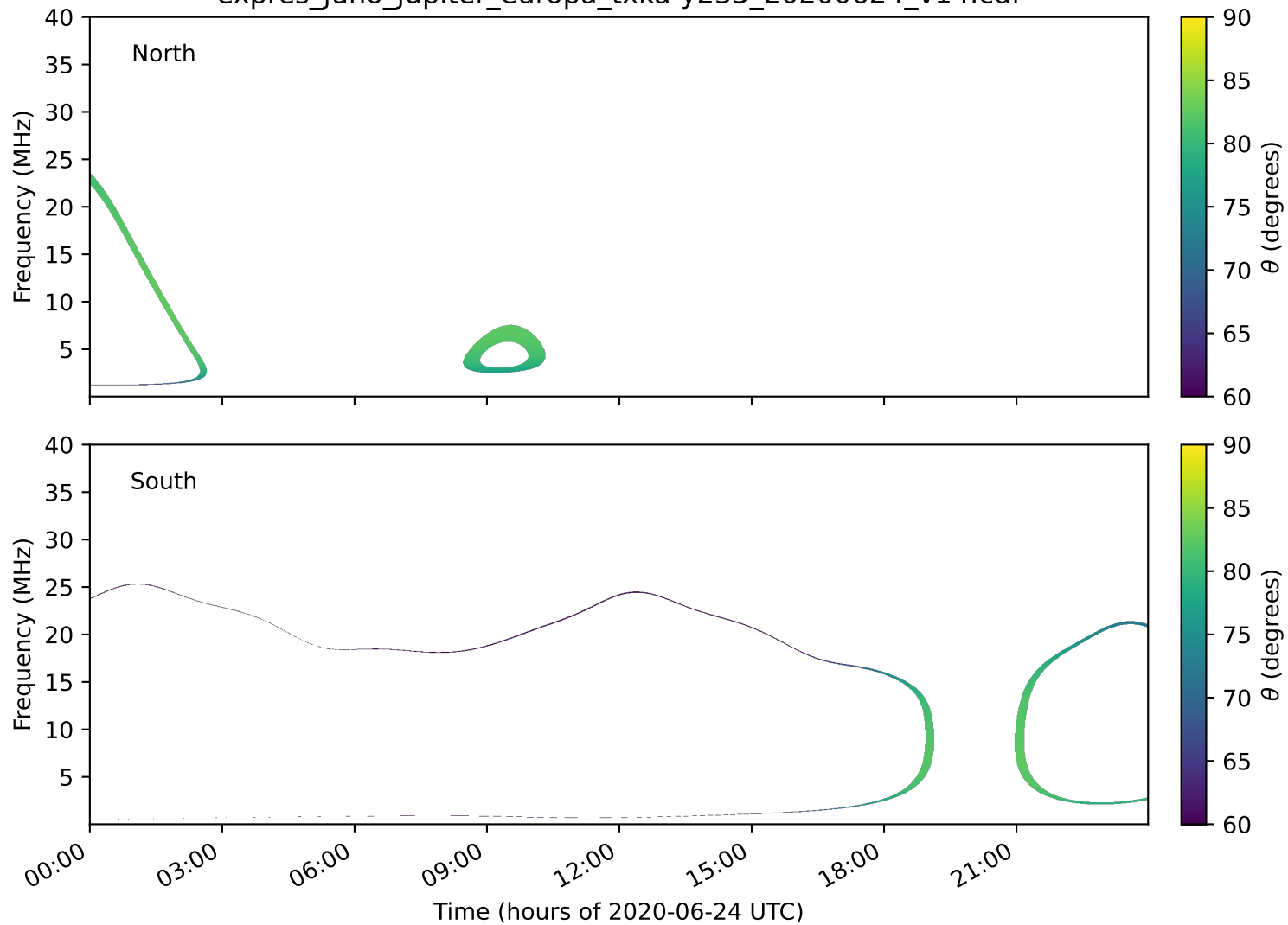
expres_juno_jupiter_europa_txka-y235_20200624_v14.cdf
