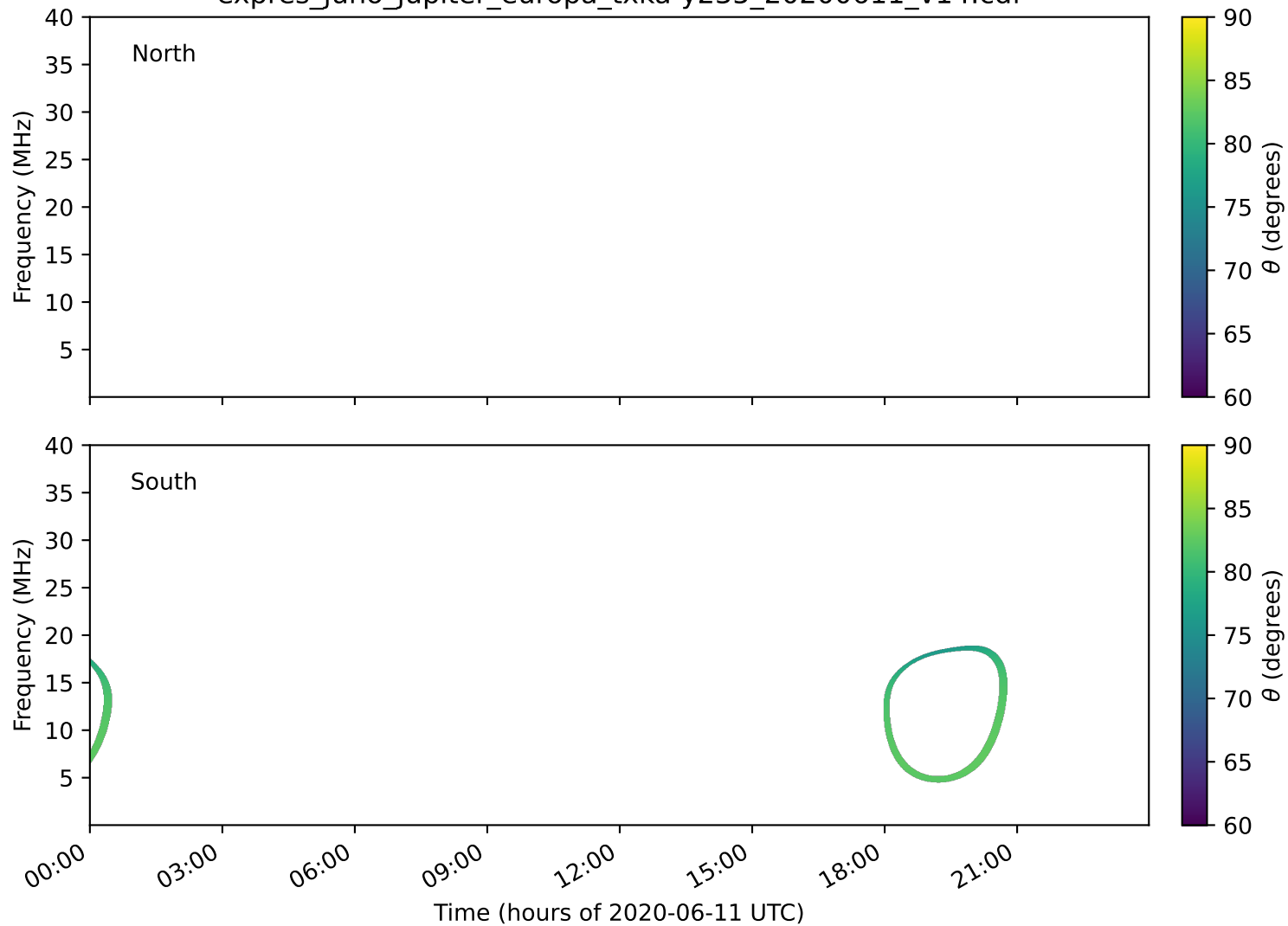
expres_juno_jupiter_europa_txka-y235_20200611_v14.cdf
