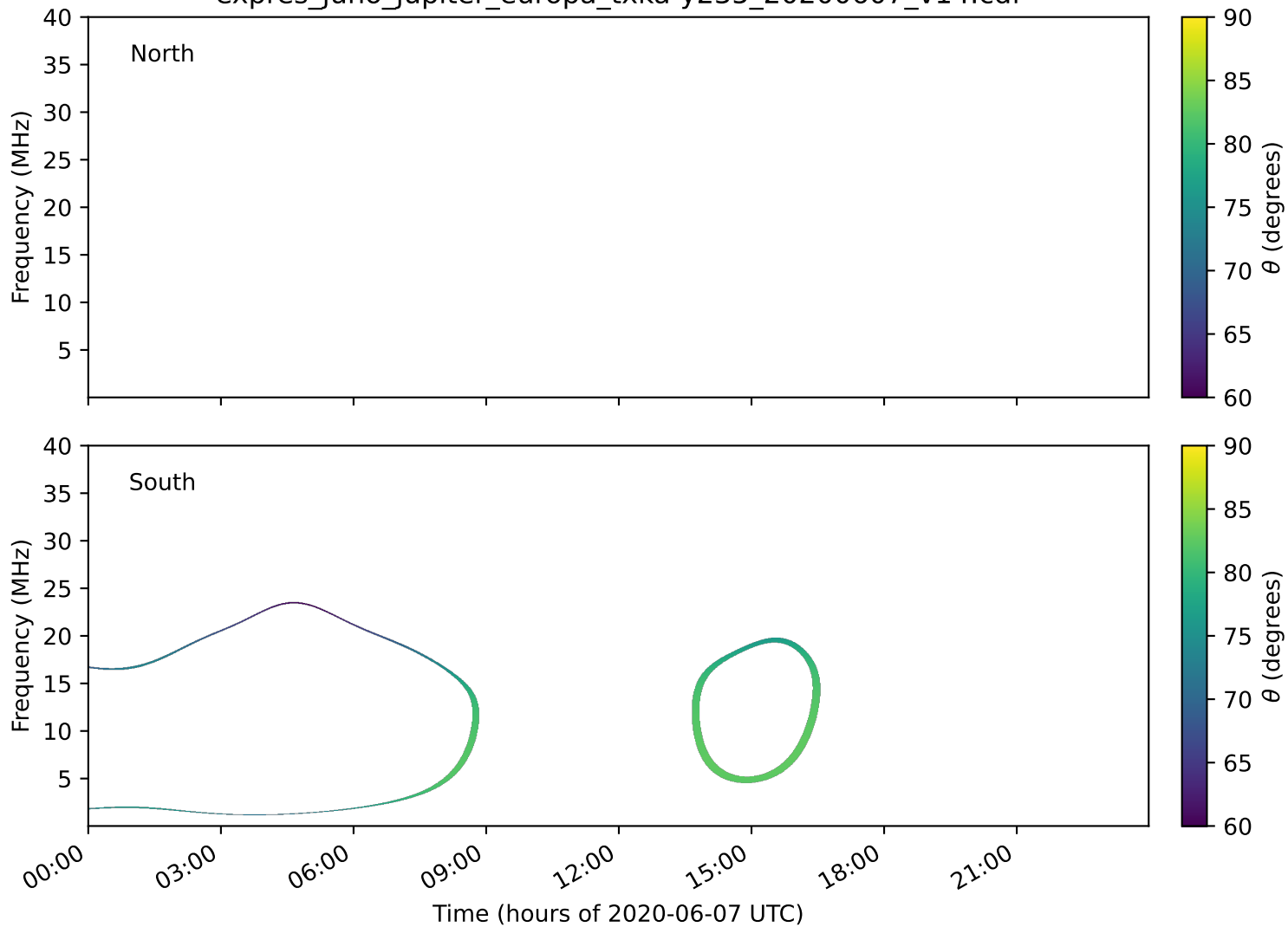
expres_juno_jupiter_europa_txka-y235_20200607_v14.cdf
