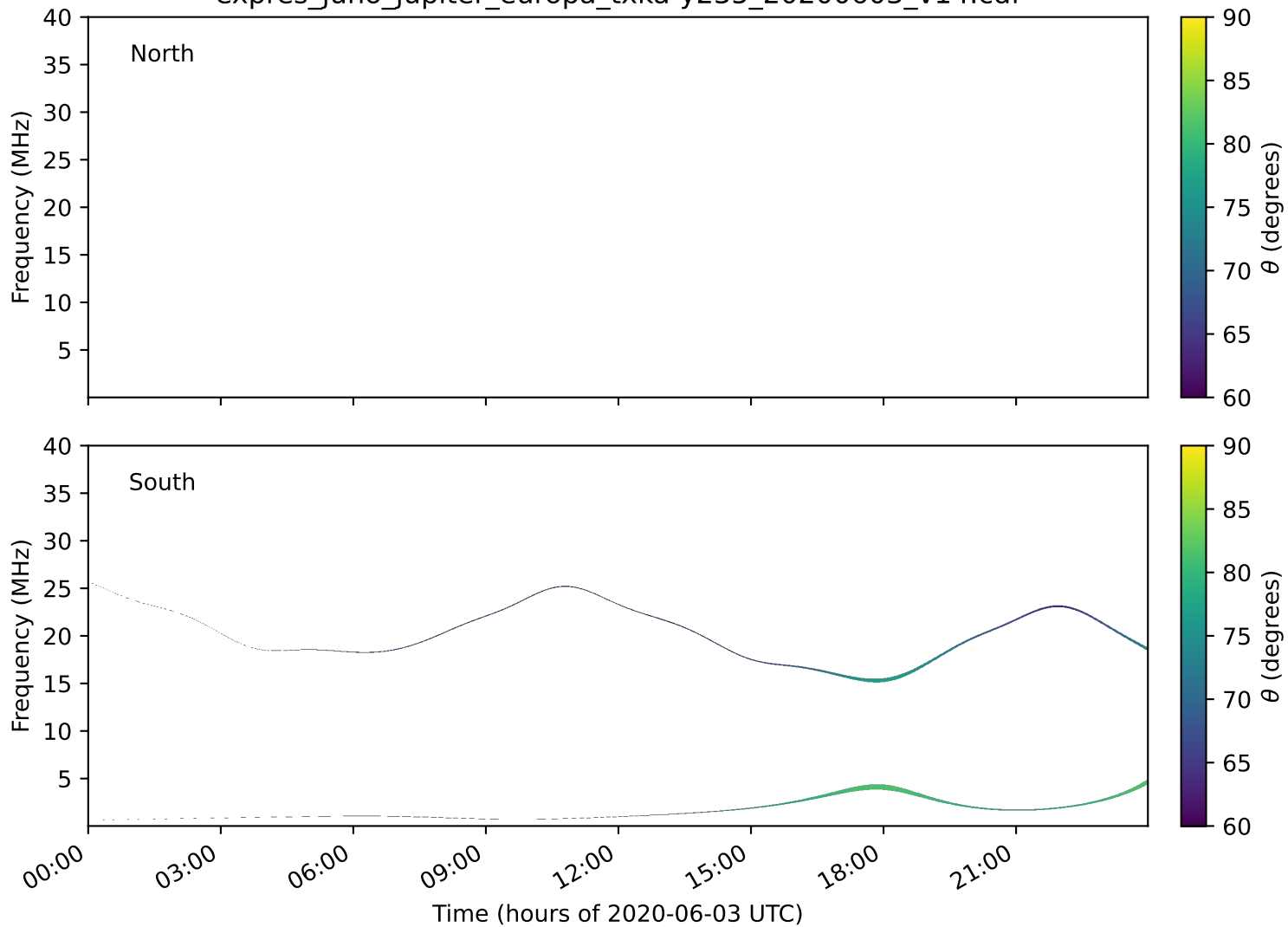
expres_juno_jupiter_europa_txka-y235_20200603_v14.cdf
