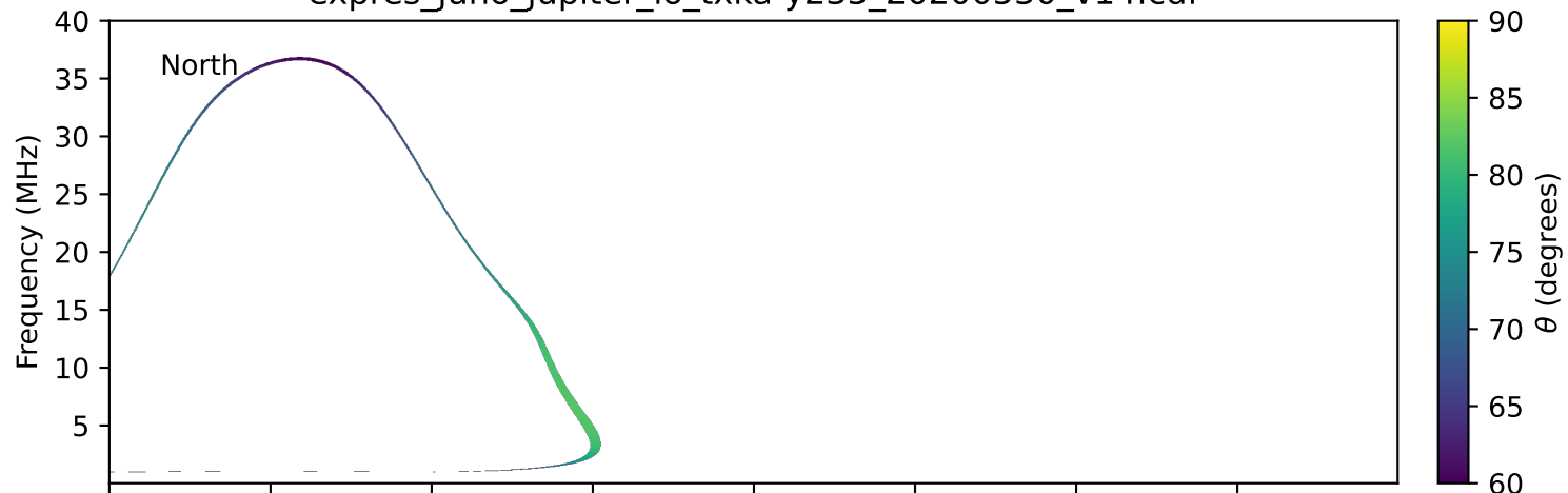
expres_juno_jupiter_io_txka-y235_20200530_v14.cdf
