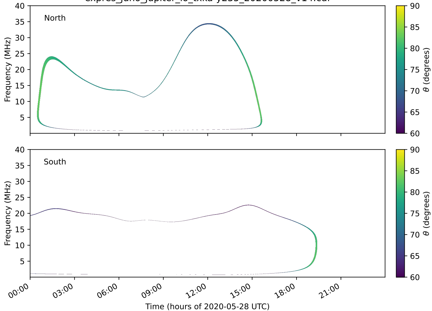
expres_juno_jupiter_io_txka-y235_20200528_v14.cdf
