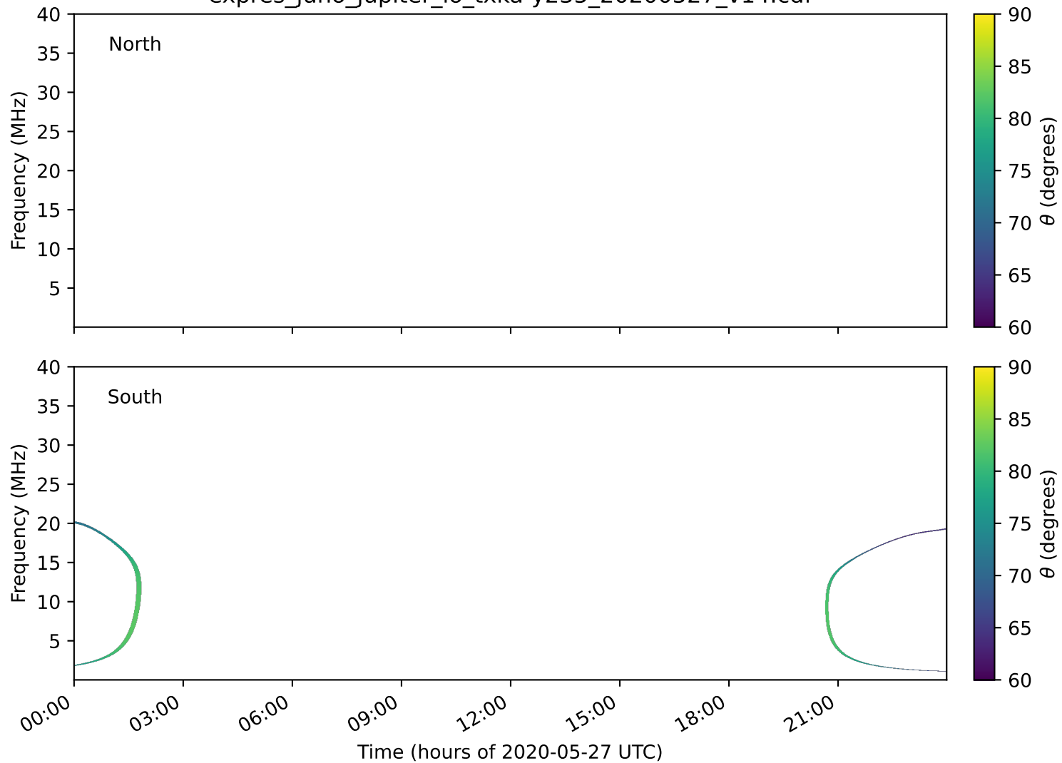
expres_juno_jupiter_io_txka-y235_20200527_v14.cdf
