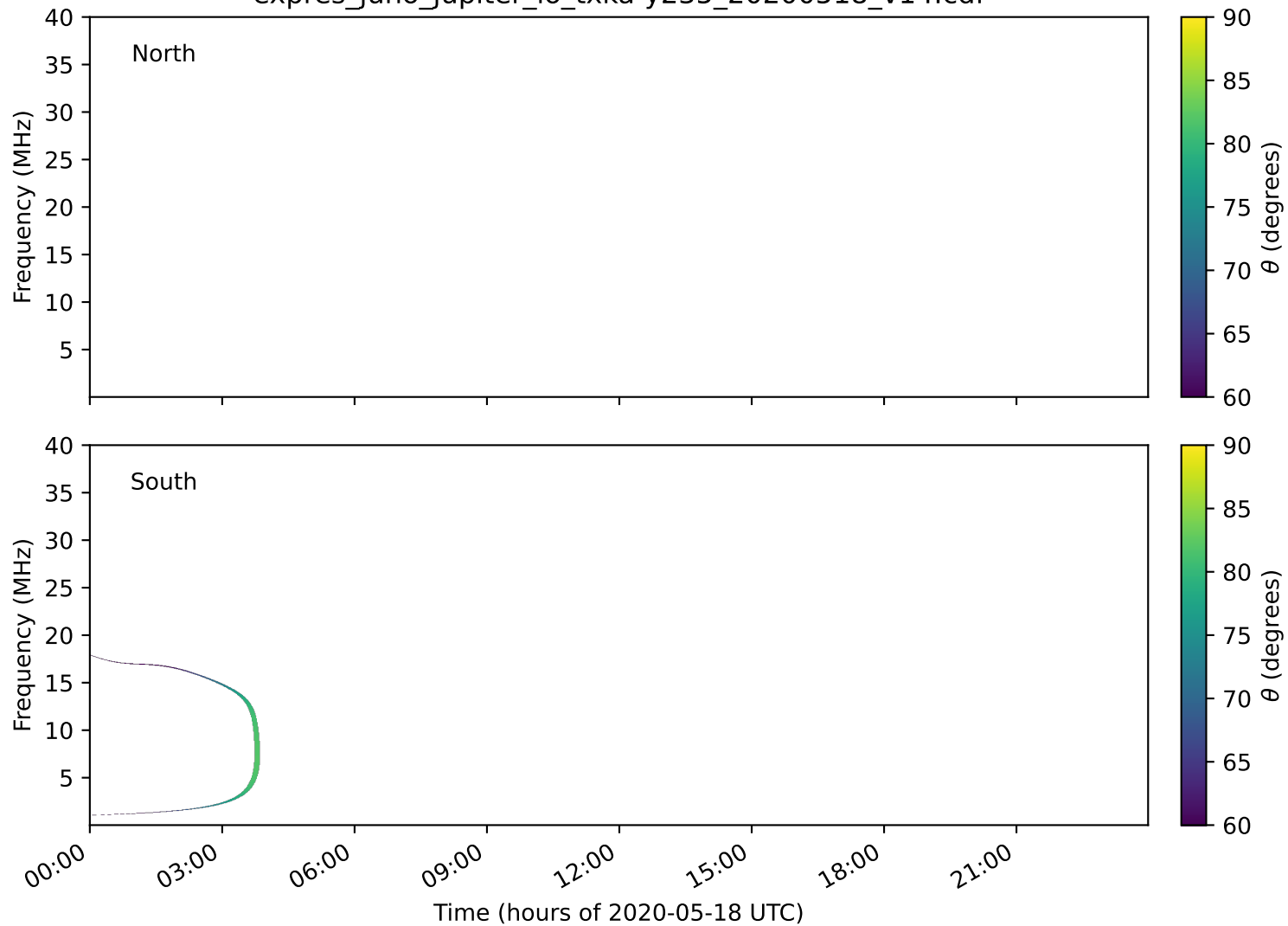
expres_juno_jupiter_io_txka-y235_20200518_v14.cdf
