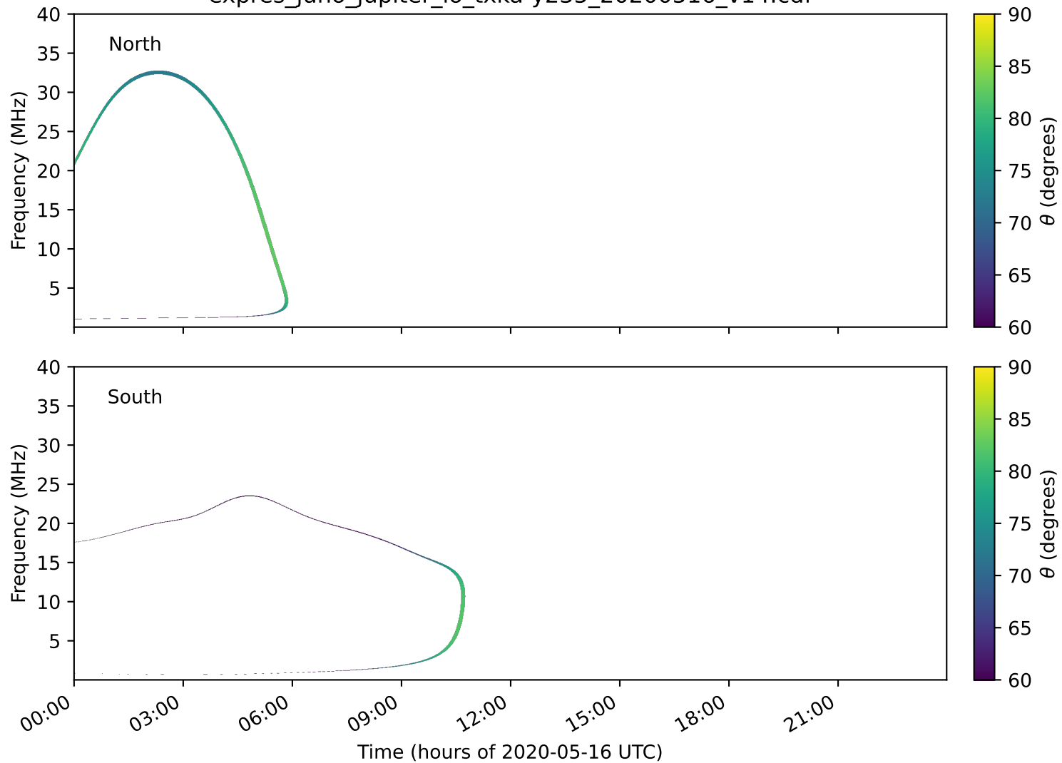
expres_juno_jupiter_io_txka-y235_20200516_v14.cdf
