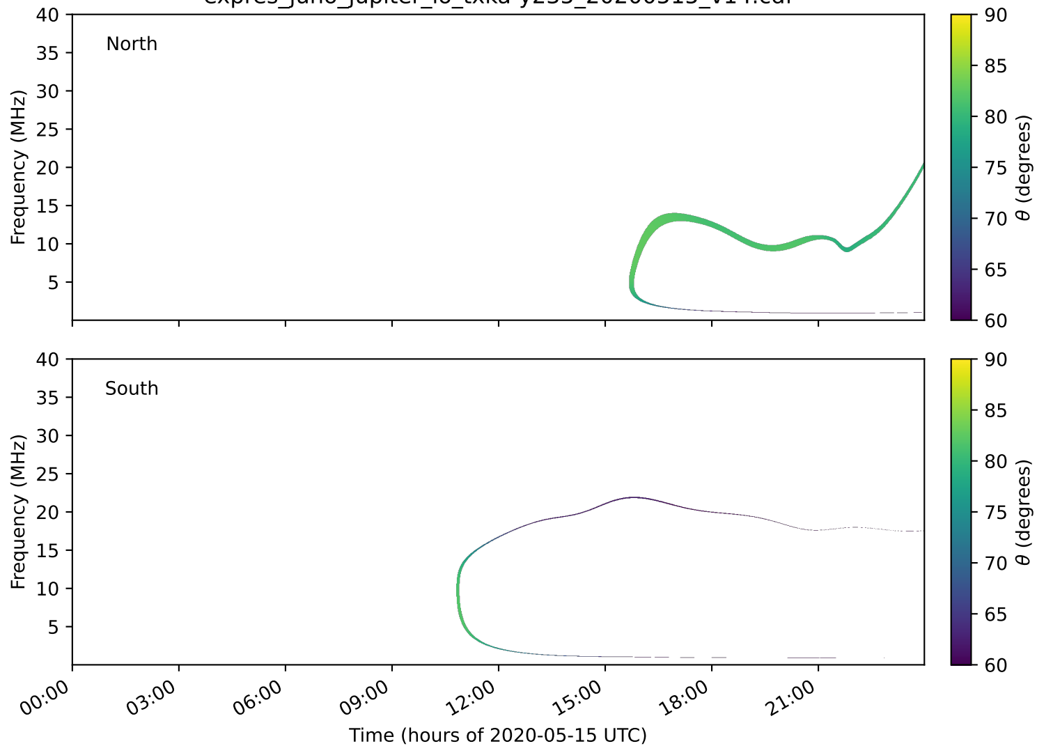
expres_juno_jupiter_io_txka-y235_20200515_v14.cdf
