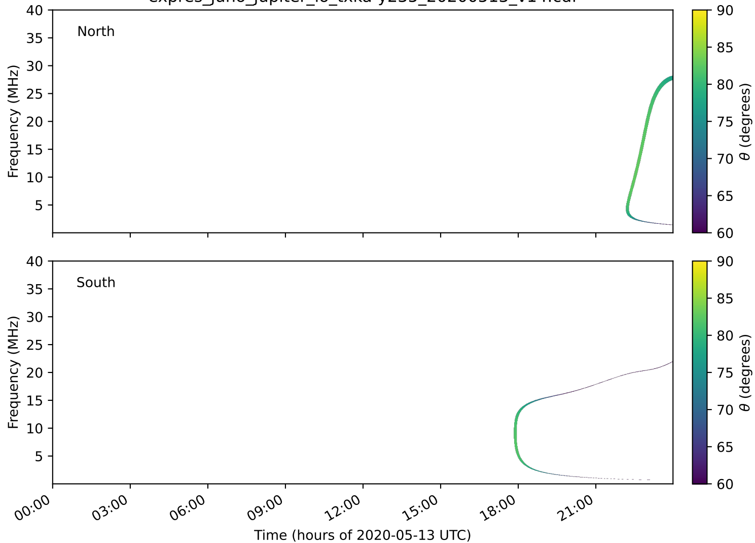
expres_juno_jupiter_io_txka-y235_20200513_v14.cdf
