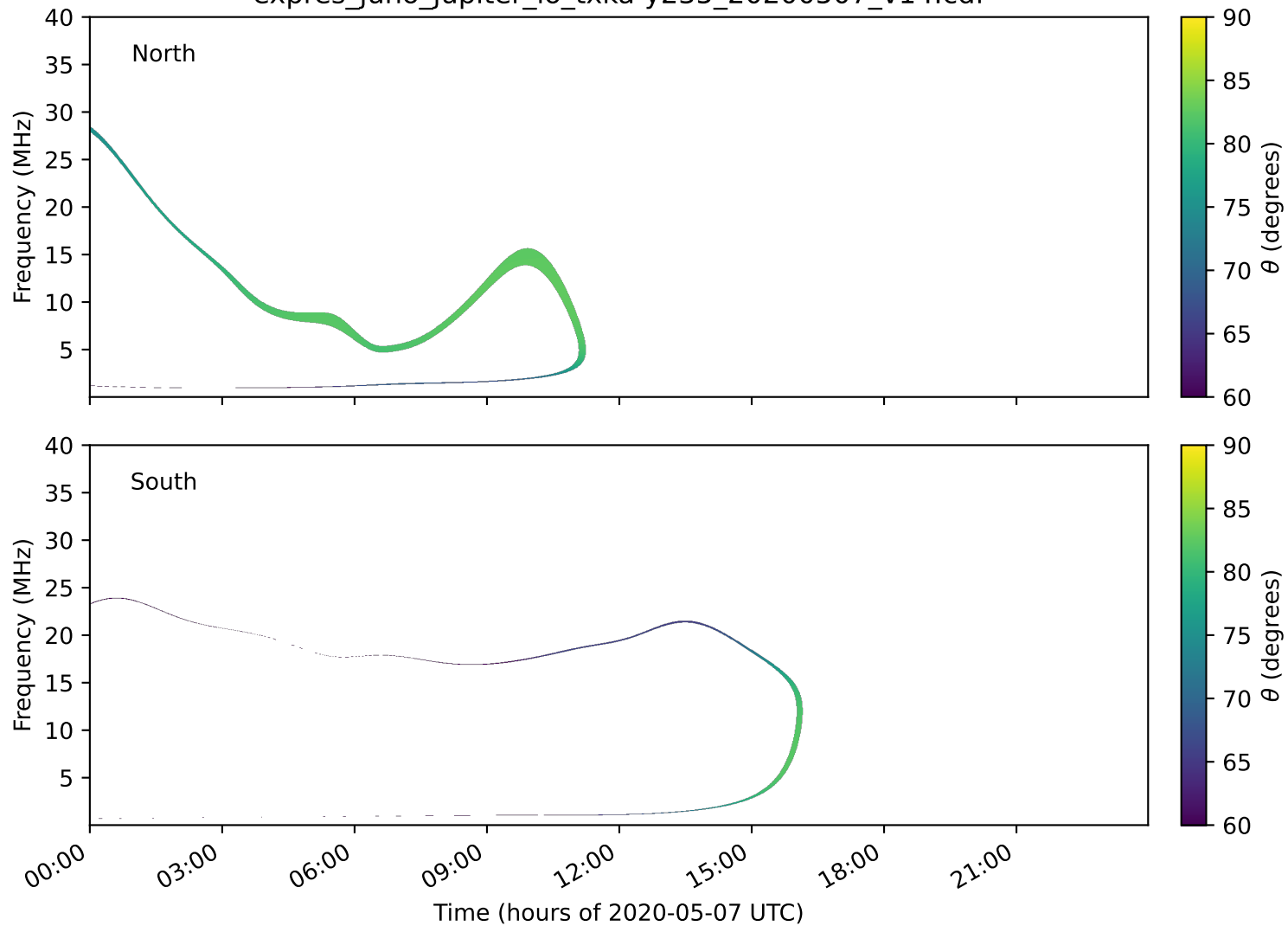
expres_juno_jupiter_io_txka-y235_20200507_v14.cdf
