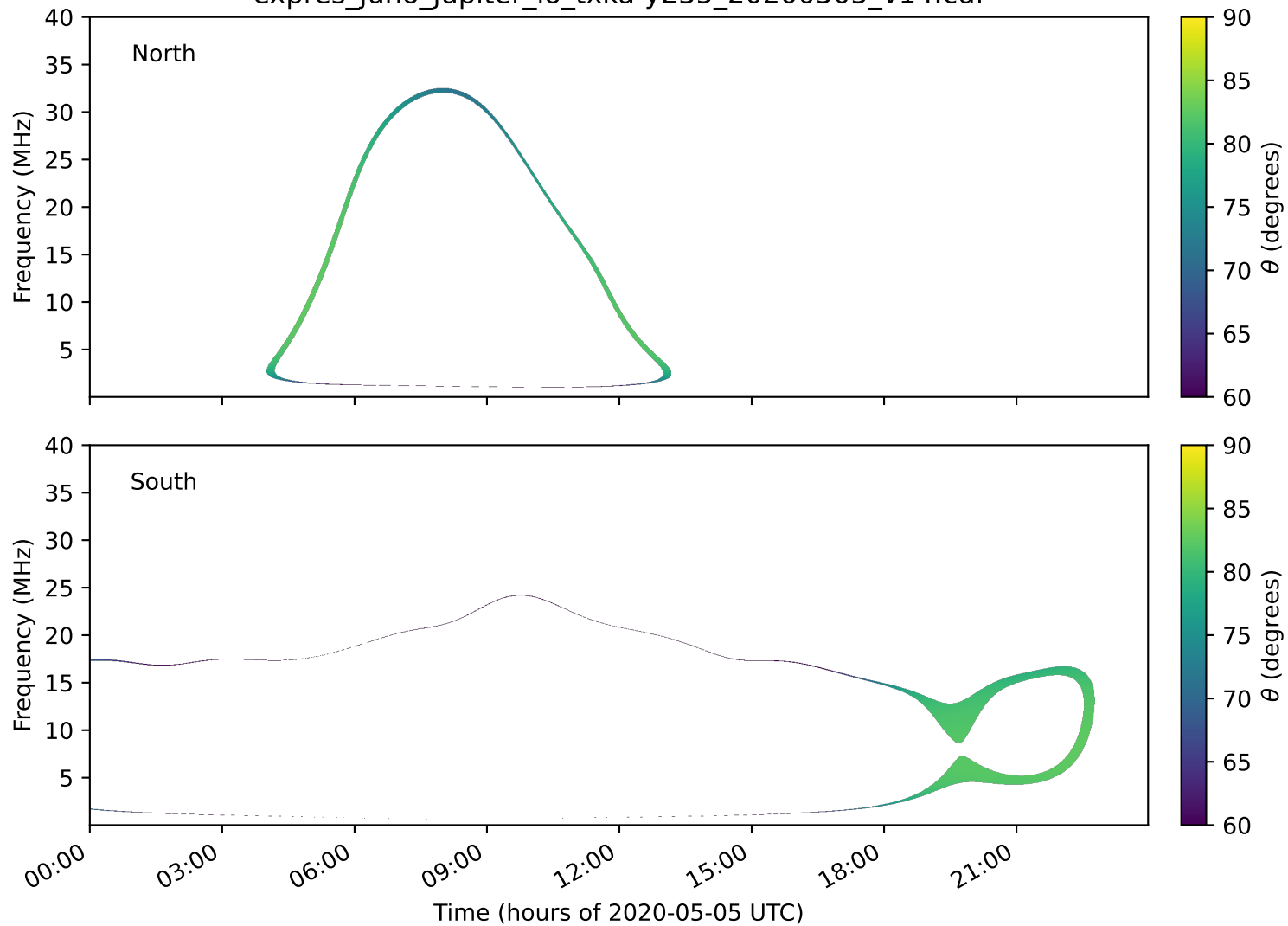
expres_juno_jupiter_io_txka-y235_20200505_v14.cdf
