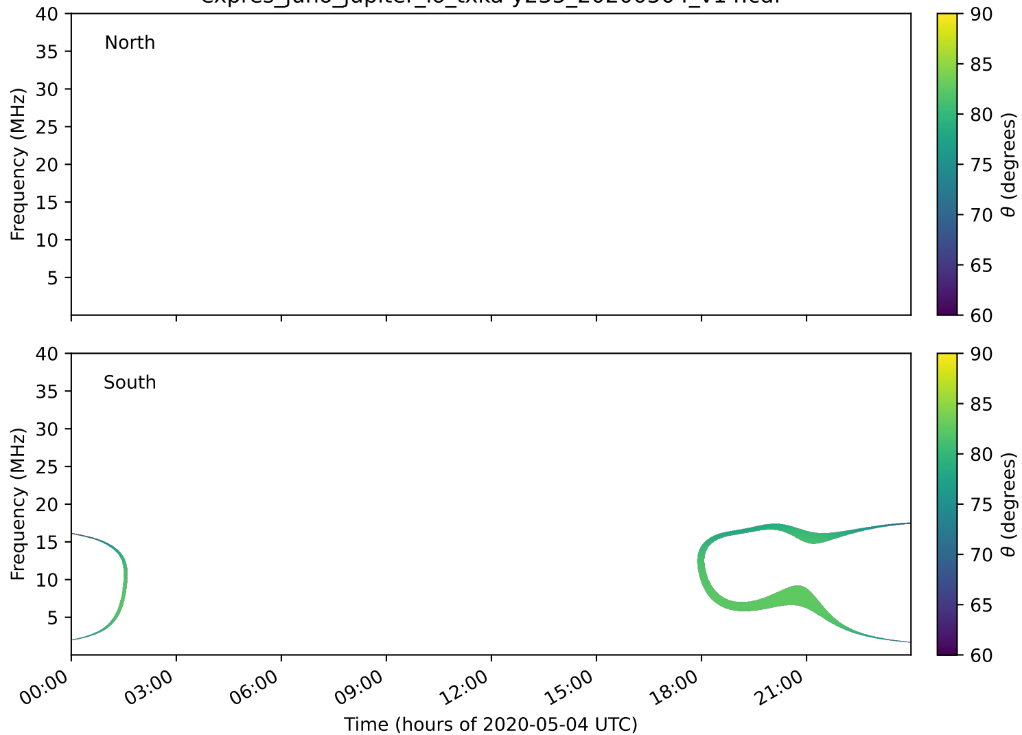
expres_juno_jupiter_io_txka-y235_20200504_v14.cdf
