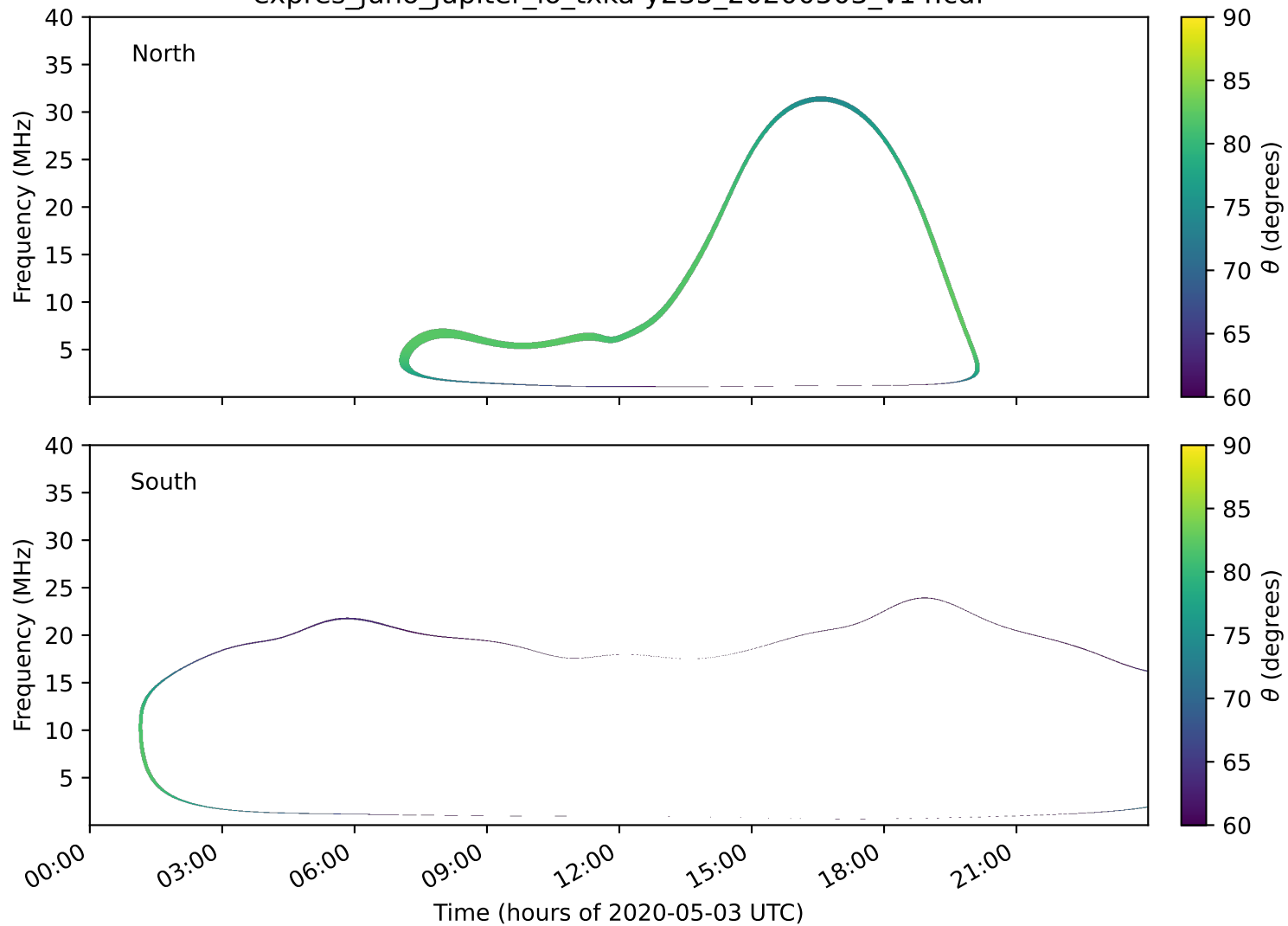
expres_juno_jupiter_io_txka-y235_20200503_v14.cdf
