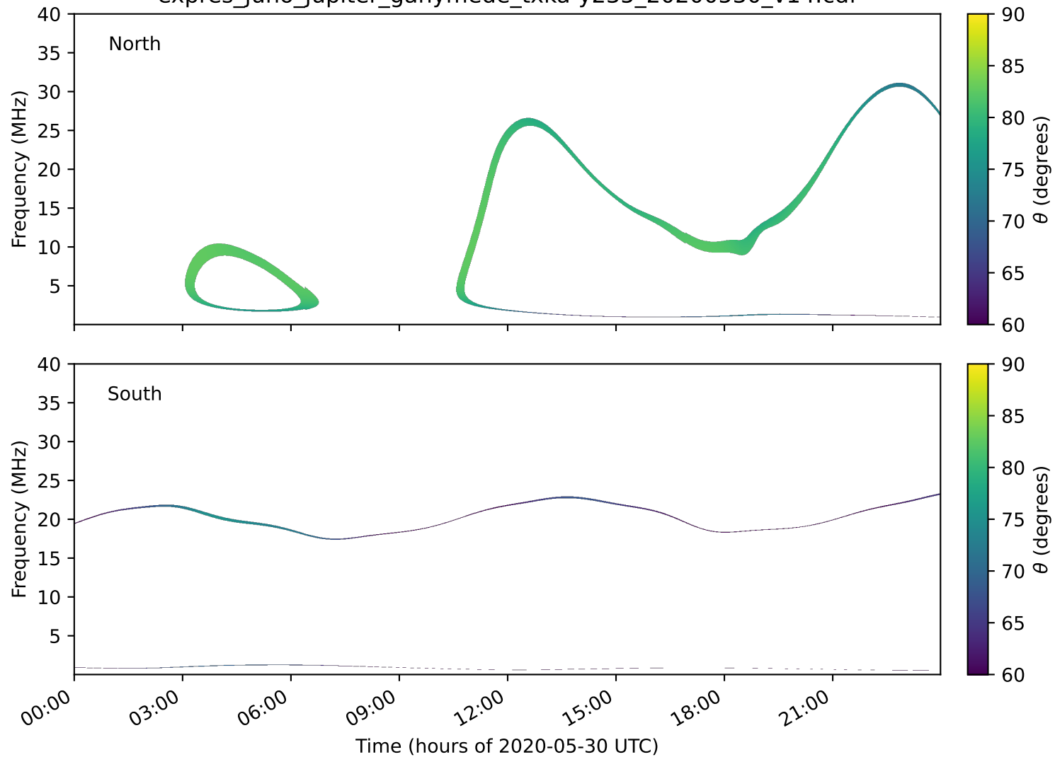
expres_juno_jupiter_ganymede_txka-y235_20200530_v14.cdf
